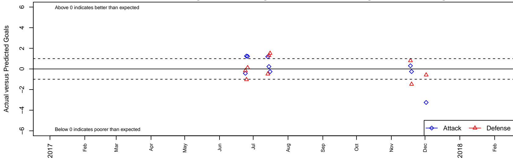
Breakers Black Wilson G99 Dots are actual minus expected GF (blue circles) and GA (red triangles). Blue line is smoothed change in attack strength. Red is smoothed change in defense strength.
